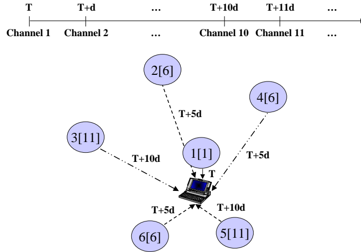
Fig. 4. SyncScan operation.
