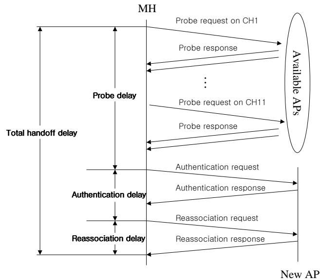
Fig. 1. Handoff message flow in IEEE 802.11 networks.
