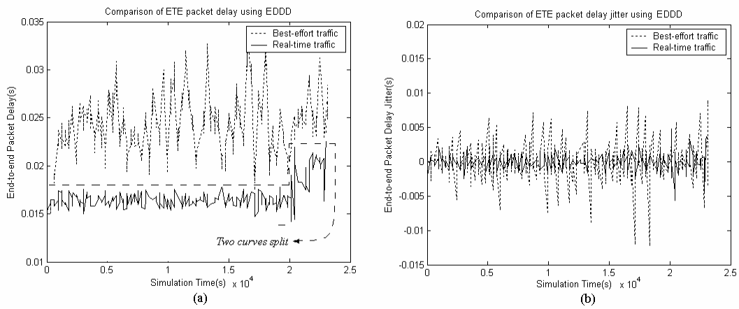
Figure 19. Comparison of ETE packet delay and delay jitter with TMR=1/2
