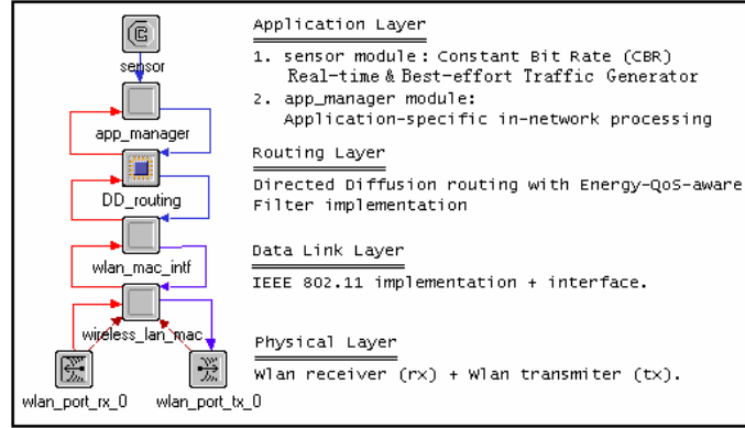
Figure 15. Sensor Node Model
