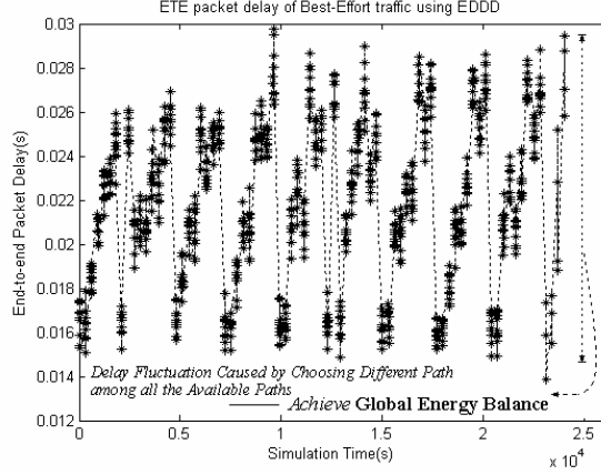
Figure 11. ETE packet delay of BE traffic using EDD
