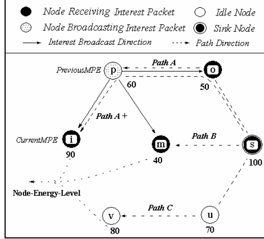
Figure. 4 Intermediate Nodes Calculate CurrentMPE When Receiving An Interest Packet
