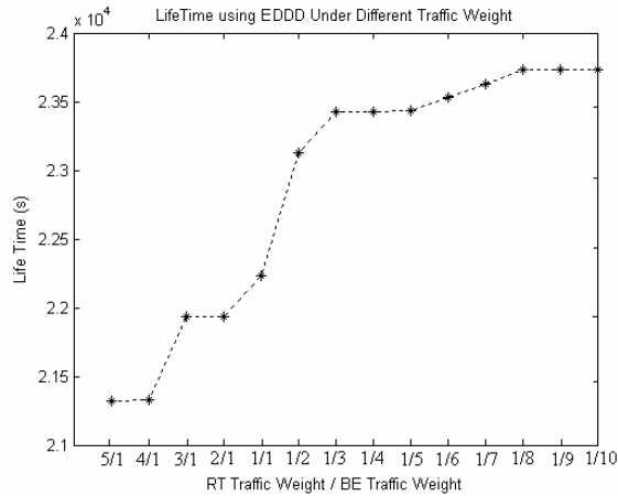
Figure 22. Comparison LifeTimeTypeII using different TMR in EDDD
