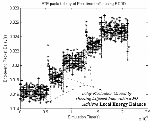
Figure 10. ETE packet delay of RT traffic using EDD
