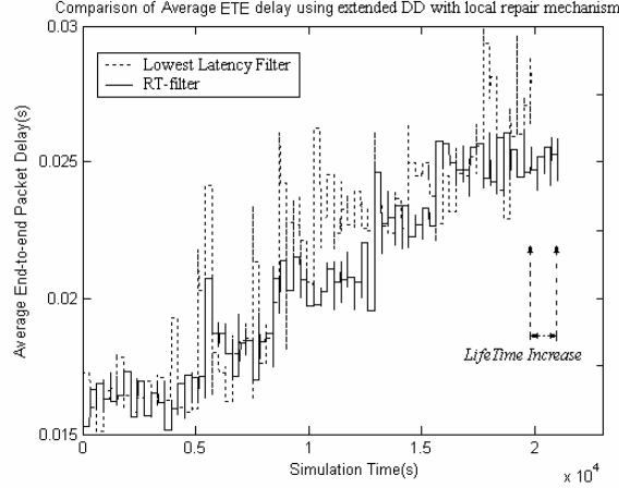
Figure 16. Comparison of ETE packet delay between Lowest Latency Filter and RT-filter
