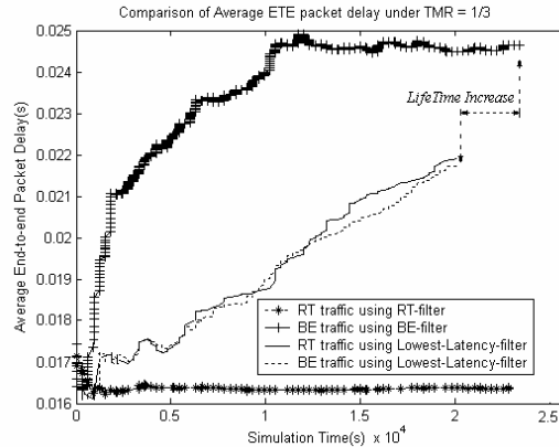
Figure 17. Comparison of ETE packet delay using tradition DD filter and RT&BE filters under TMR=1/3
