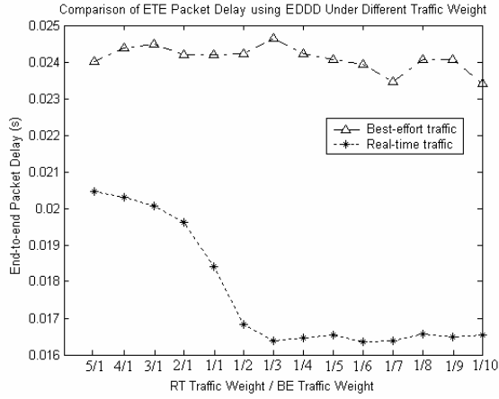
Figure 21. Comparison average ETE packet delay using different TMR in EDDD
