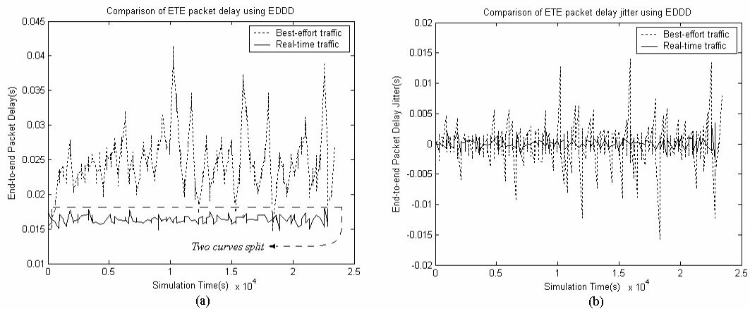
Figure 20. Comparison of ETE packet delay and delay jitter with TMR=1/3
