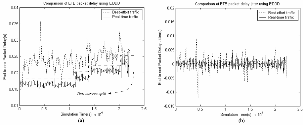
Figure 18. Comparison of ETE packet delay and delay jitter with TMR=1/1
