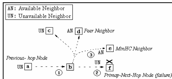
Figure 12. Intermediate Node Chooses Second Best Neighbor For RT packet
