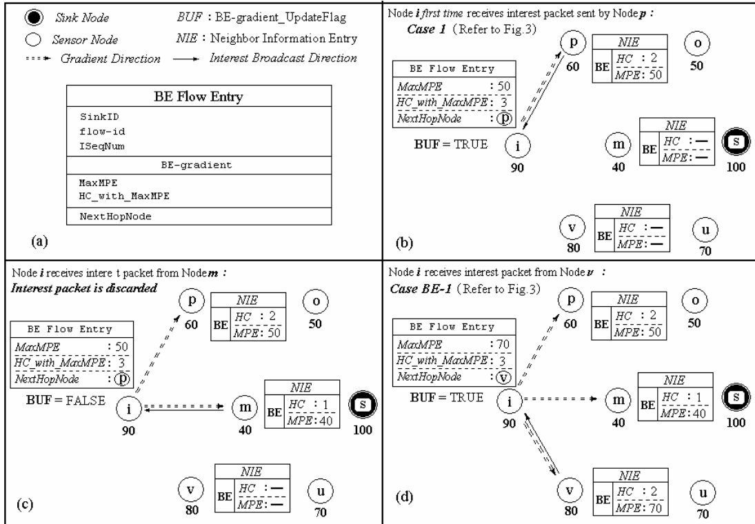
Figure 5. Intermediate Nodes setup a BE-gradient and update a BE-flow-entry when receiving interest packet with BUF set
