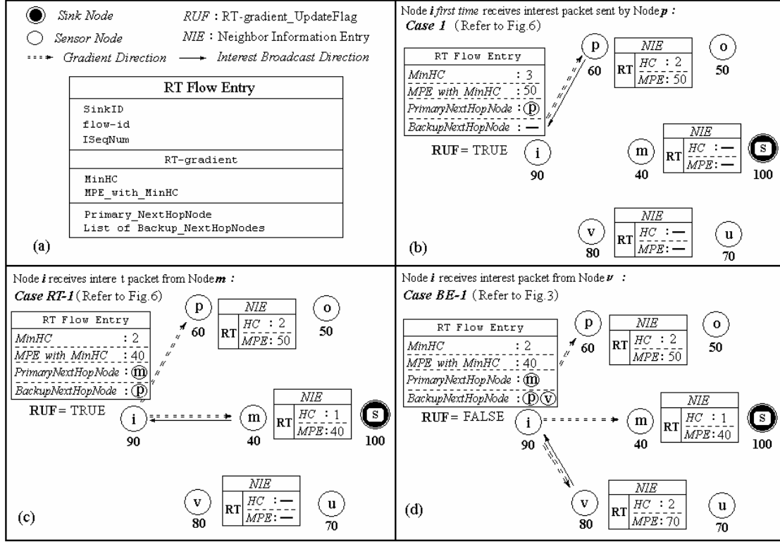
Figure 7. Intermediate Nodes Setup RT-gradients and update RT-flow-entry when receiving interest packets with RUF set
