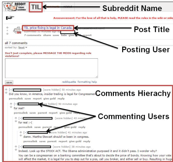
Figure 1: A post with its associated comments in the subreddit “Today I Learned (TIL)” is illustrated.
