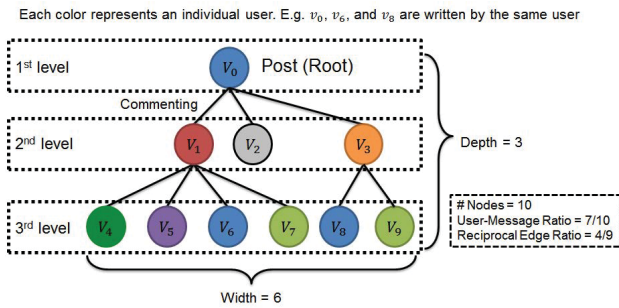
Figure 3: A comment tree is illustrated for a post that has 9 comments.
