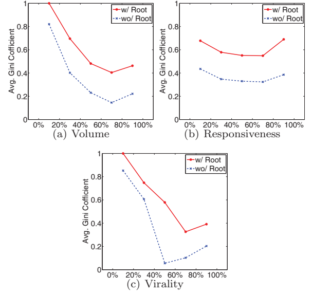
Figure 10: Average of Gini coefficients of comment trees are plotted as the volume, responsiveness, and virality increase.
