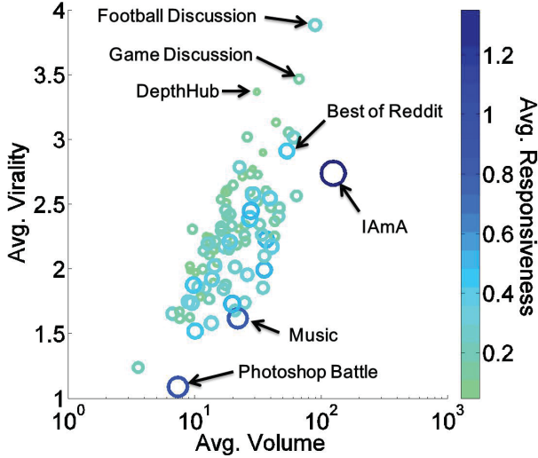
Figure 13: We map subreddits by calculating the average values of their trees in terms of the volume, responsiveness, and virality.
