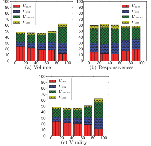
Figure 12: Contribution ratios of four user role types are plotted.
