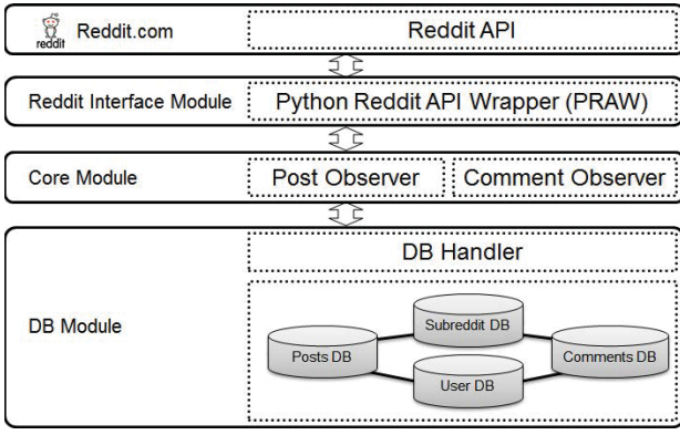
Figure 2: The architecture of the Reddit measurement system is depicted.
