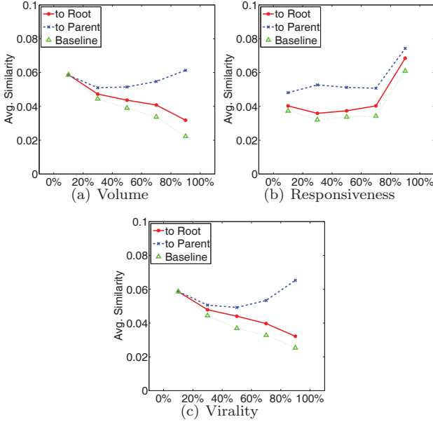
Figure 9: The relevance among messages of a comment tree is plotted.
