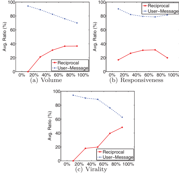
Figure 11: Reciprocal edge ratio and User-Message Ratio are plotted.
