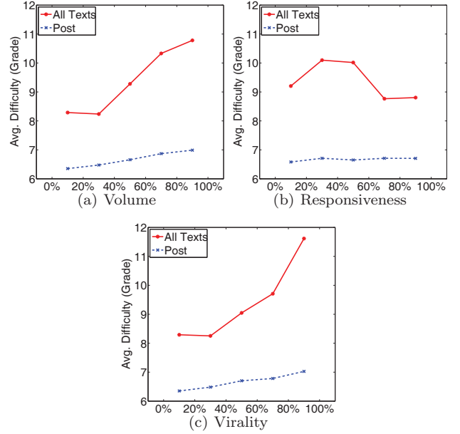
Figure 8: The average difficulties of trees and posts are plotted as the volume, responsiveness, and virality increase.
