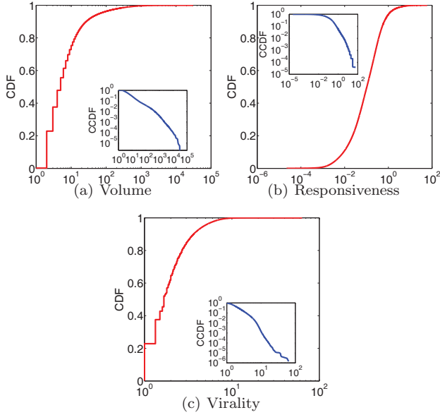
Figure 5: Distributions of volume, responsiveness, and virality of comment trees are plotted for all the comment trees.
