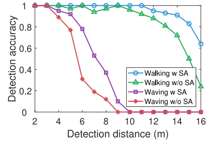
Fig. 14. Detection distance of different activities.
