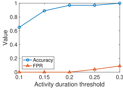
Fig. 13. Activity detection accuracy and FPR in different duration threshold settings.
