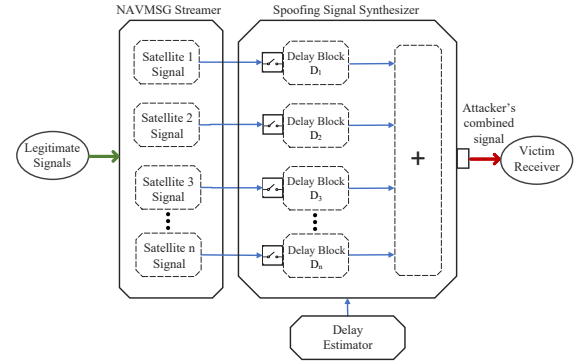
Figure 3: Signal processing pipeline. i) NAVMSG streamer, ii) the delay estimator, and iii) signal synthesizer module.
