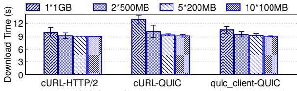
Figure 12: Parallel download experiments (instances of cURL or quic_client download 1 GB of files in total).
