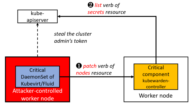
Figure 8: The potential risk of Kubewarden. The attacker can leverage the DaemonSet of other apps to force the Kubewarden’s critical component to run on the attacker-controlled node, then he/she can use its excessive permission to get the cluster admin’s token.
