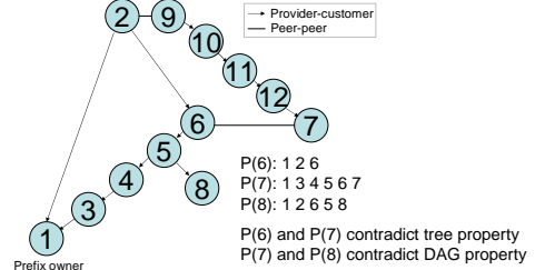
Figure 2: An example AS topology where collapsing the victim AS 1's paths in its vPath results in a graph containing a loop.
