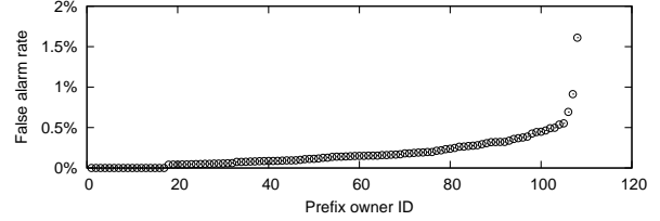
Figure 5: False positive ratios of the 108 PlanetLab hosts during the 25-day period. Detection threshold was set to 10.
