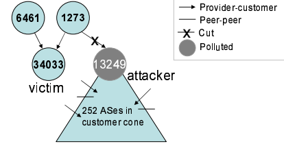
Figure 4: An example hijacking instance with small |\Omega| .
