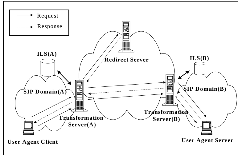
Figure 3: The Proposed New SIP Architecture.
