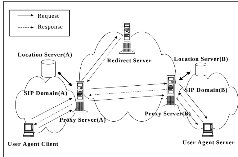
Figure 1: SIP architecture.
